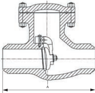
BUTT-WELD END
