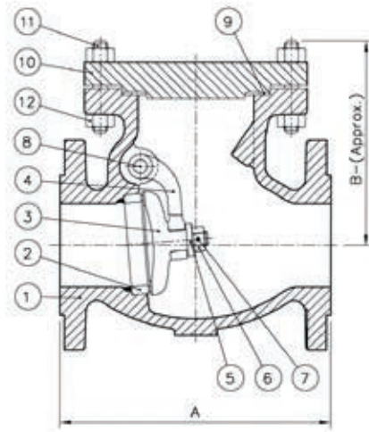
FLANGED END
