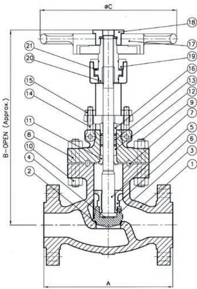
FLANGED END
