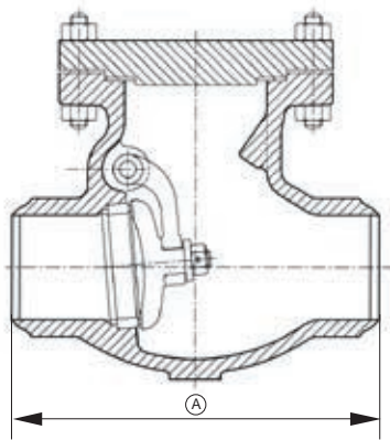
BUTT-WELD END
