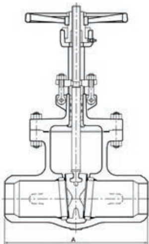
BUTT-WELD END
