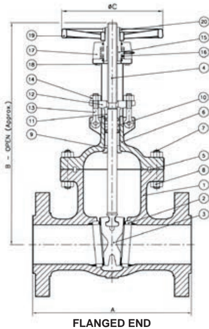
FLANGED END
